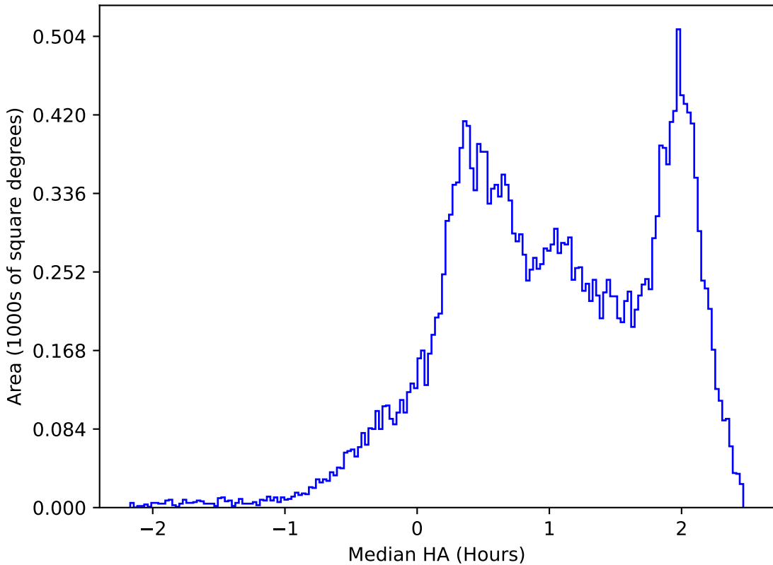
ddf_acor_sf15_lsf40_lsr20_v3.4_10yrs All sky z band: Median HA
