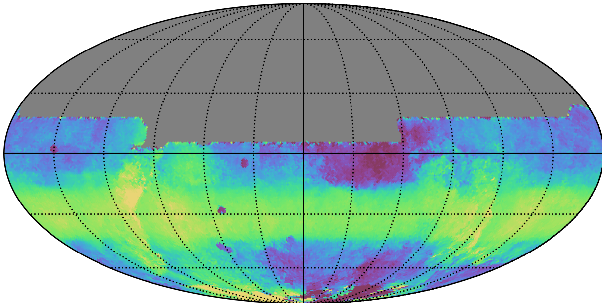
ddf_acor_sf15_lsf40_lsr20_v3.4_10yrs All sky y band: Median HA
