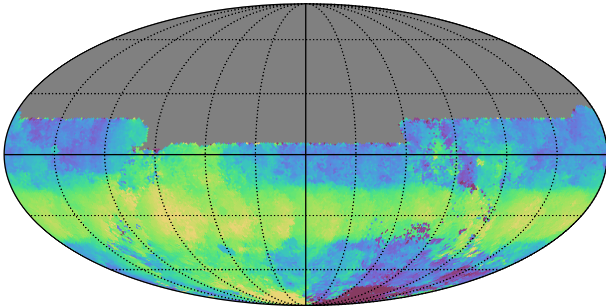
ddf_acor_sf15_lsf40_lsr20_v3.4_10yrs All sky u band: Median HA
