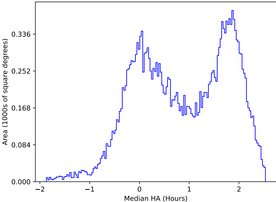
ddf_acor_sf15_lsf40_lsr20_v3.4_10yrs All sky u band: Median HA
