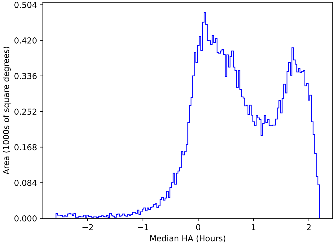
ddf_acor_sf15_lsf40_lsr20_v3.4_10yrs All sky r band: Median HA
