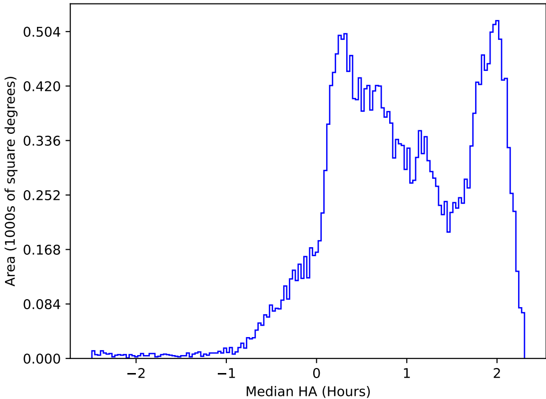
ddf_acor_sf15_lsf40_lsr20_v3.4_10yrs All sky i band: Median HA
