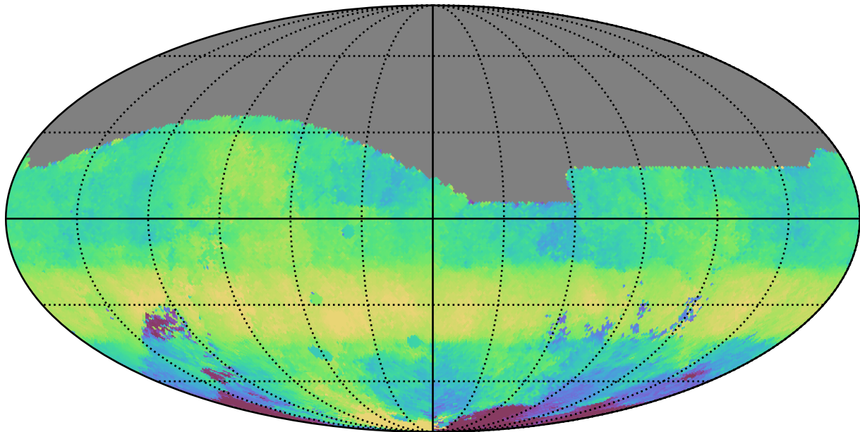
ddf_acor_sf15_lsf40_lsr20_v3.4_10yrs All sky g band: Median HA
