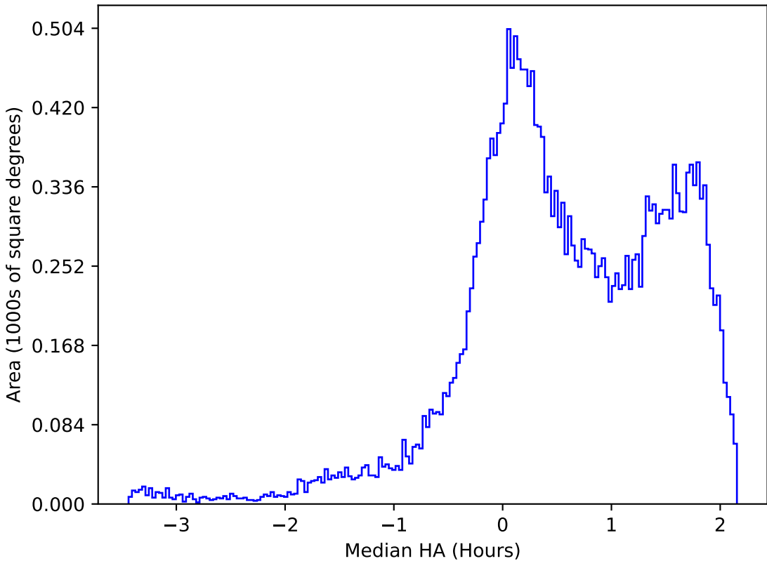
ddf_acor_sf15_lsf40_lsr20_v3.4_10yrs All sky g band: Median HA
