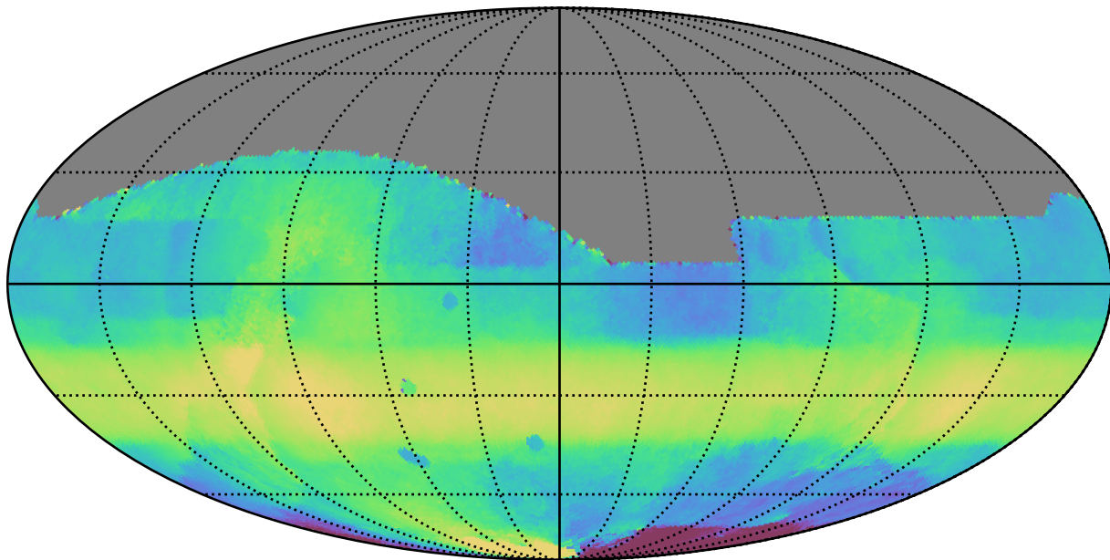
ddf_acor_sf15_lsf40_lsr20_v3.4_10yrs All sky all bands: Median HA
