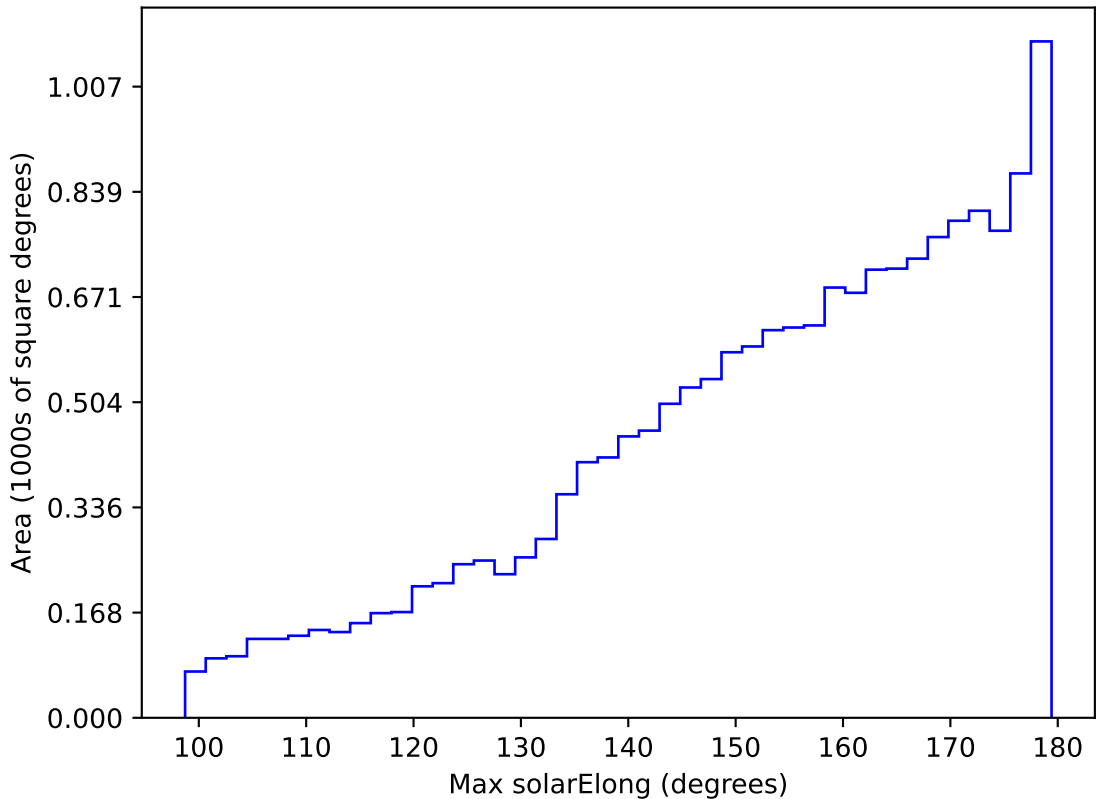
ddf_acor_sf15_lsf40_lsr20_v3.4_10yrs WFD z band: Max solarElong
