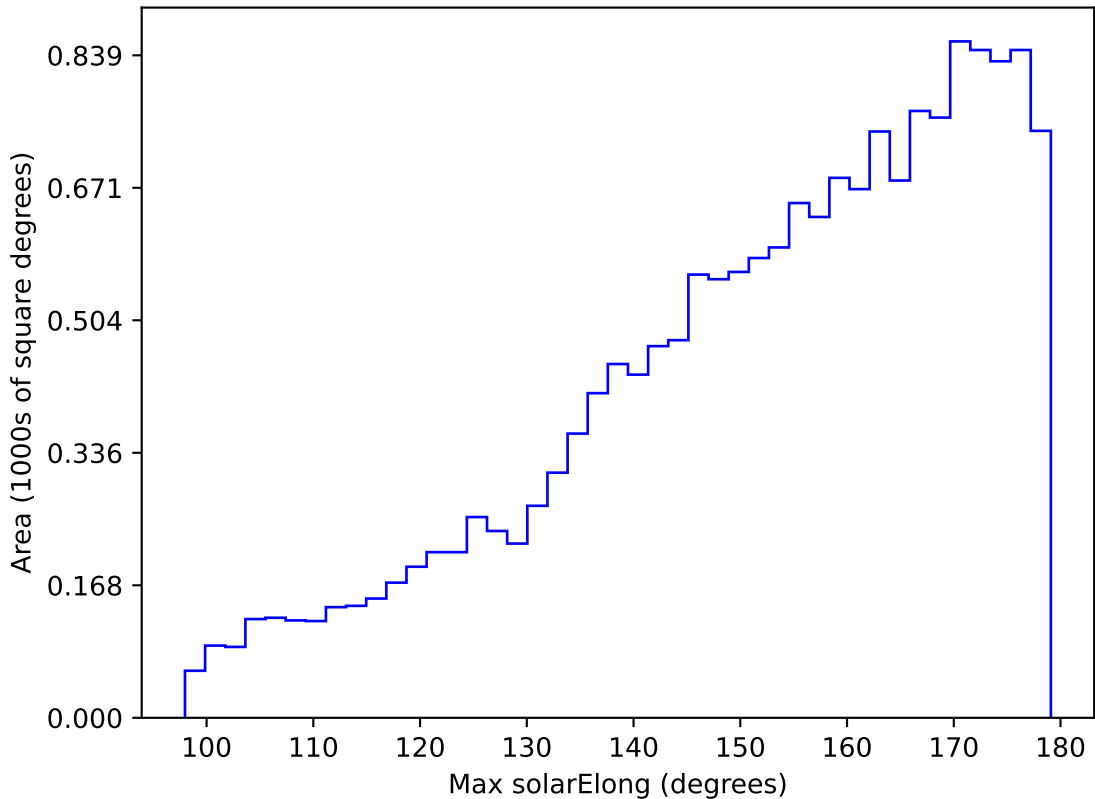
ddf_acor_sf15_lsf40_lsr20_v3.4_10yrs WFD u band: Max solarElong
