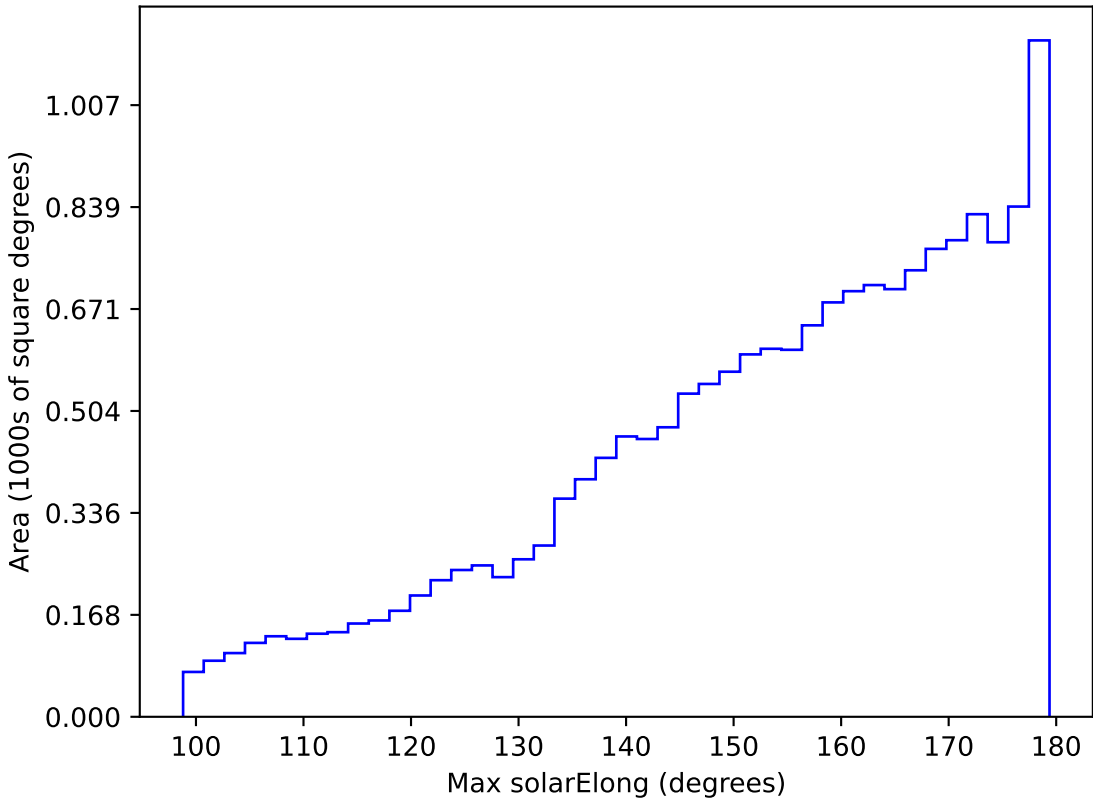
ddf_acor_sf15_lsf40_lsr20_v3.4_10yrs WFD i band: Max solarElong
