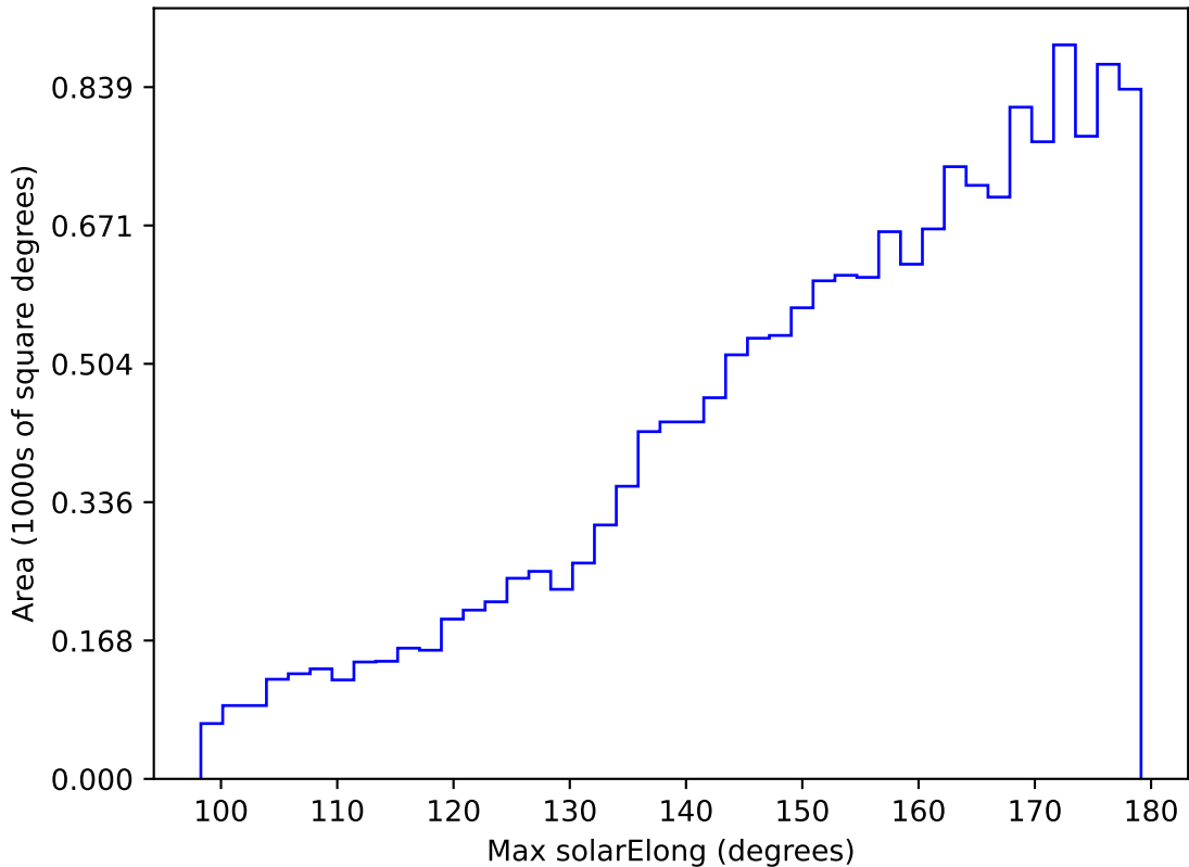
ddf_acor_sf15_lsf40_lsr20_v3.4_10yrs WFD g band: Max solarElong
