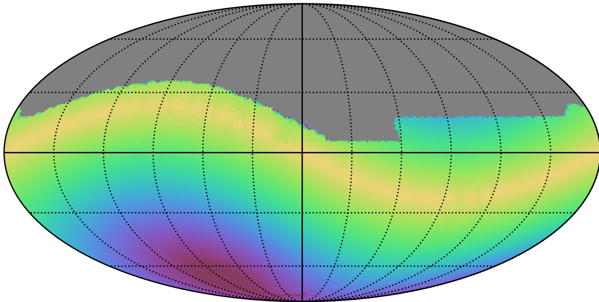
ddf_acor_sf15_lsf40_lsr20_v3.4_10yrs All sky r band: Max solarElong
