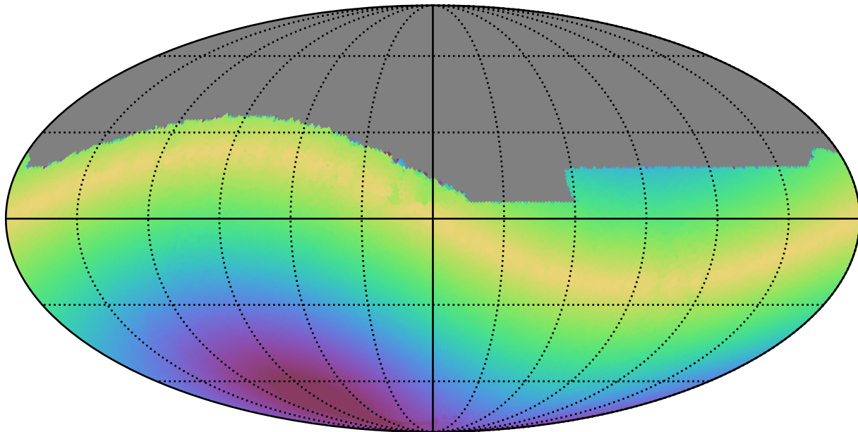
ddf_acor_sf15_lsf40_lsr20_v3.4_10yrs All sky i band: Max solarElong
