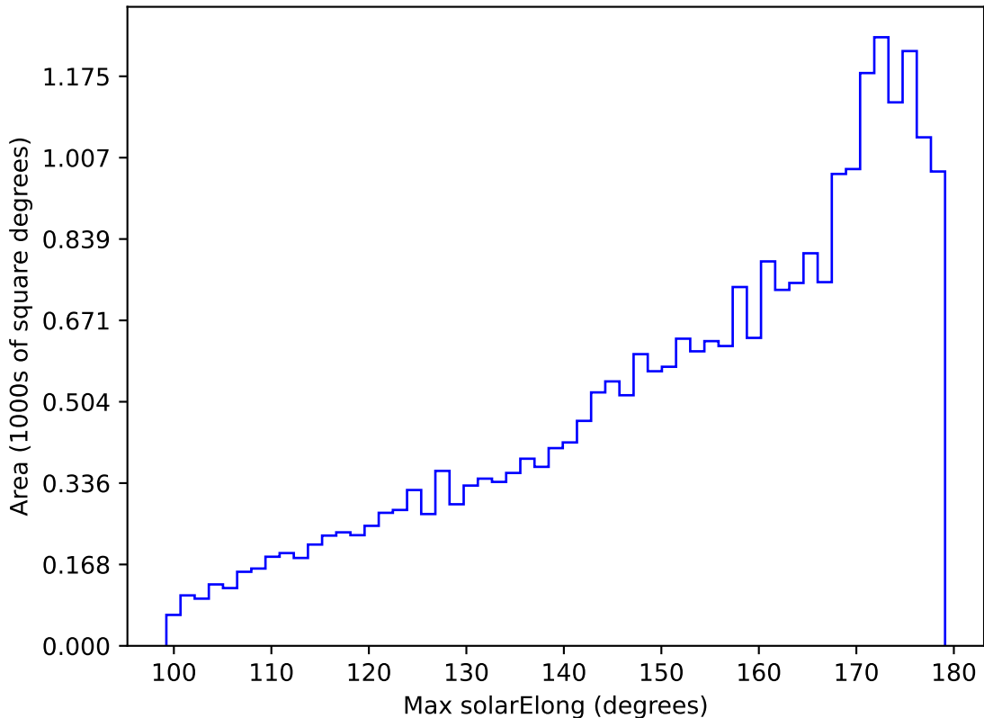
ddf_acor_sf15_ls40_lsr20_v3.4_10yrs All sky g band: Max solarElong
