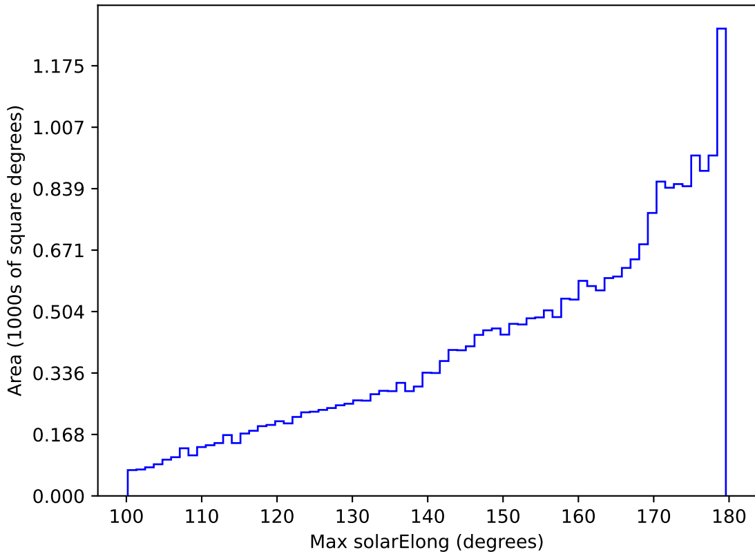
ddf_acor_sf15_lsf40_lsr20_v3.4_10yrs All sky all bands: Max solarElong
