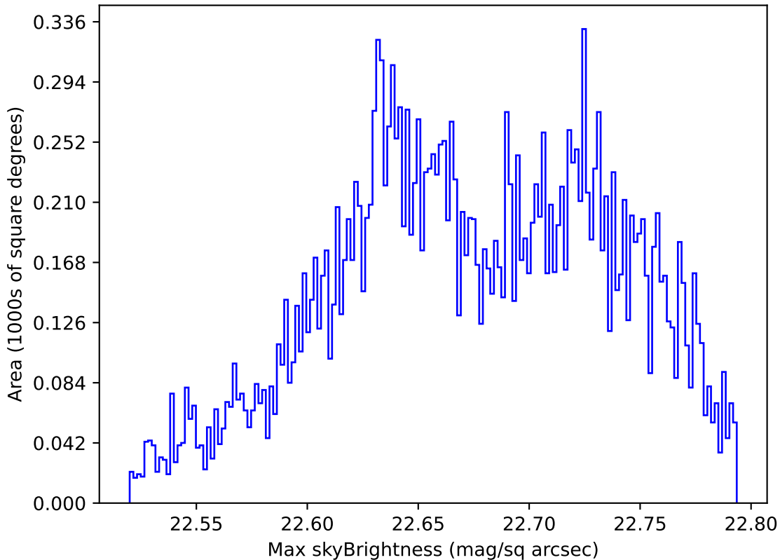
ddf_acor_sf15_lsf40_lsr20_v3.4_10yrs Yr 1 u band: Max skyBrightness
