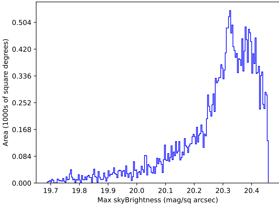
ddf_acor_sf15_lsf40_lsr20_v3.4_10yrs Yr 1 i band: Max skyBrightness
