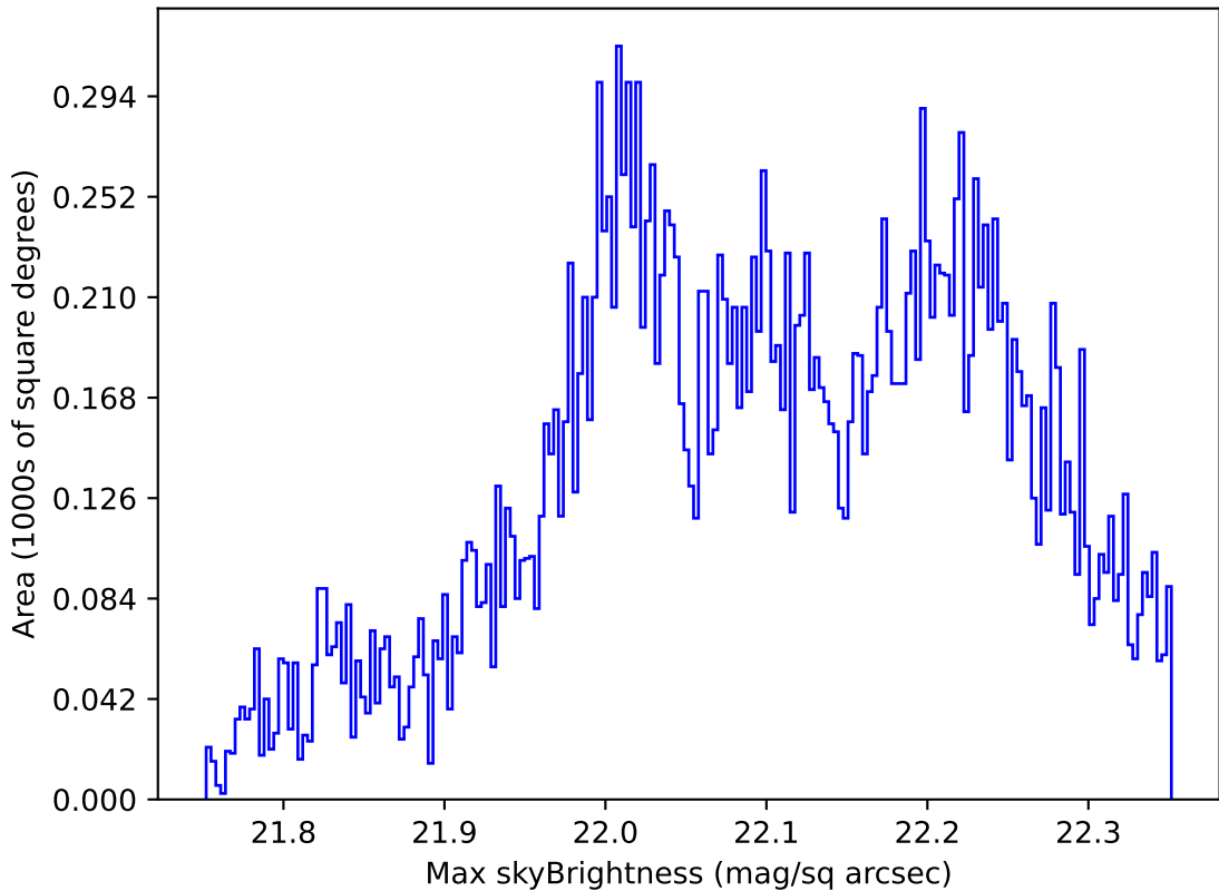
ddf_acor_sf15_lsf40_lsr20_v3.4_10yrs Yr 1 g band: Max skyBrightness
