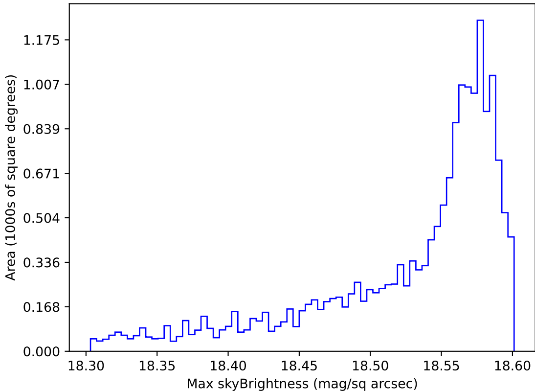
ddf_acor_sf15_lsf40_lsr20_v3.4_10yrs WFD y band: Max skyBrightness
