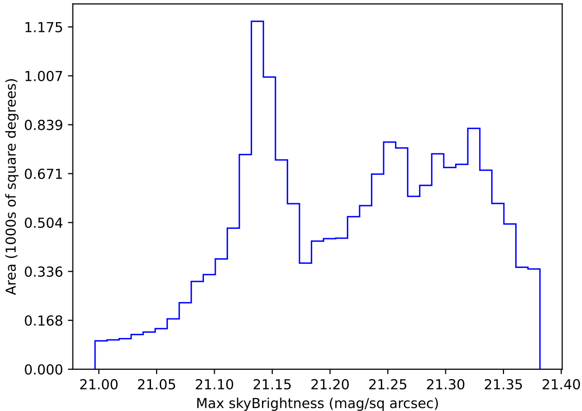
ddf_acor_sf15_lsf40_lsr20_v3.4_10yrs WFD r band: Max skyBrightness
