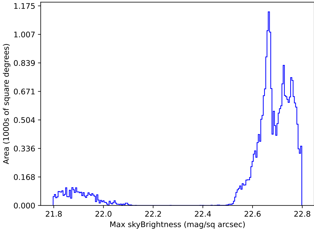
ddf_acor_sf15_lsf40_lsr20_v3.4_10yrs All sky all bands: Max skyBrightness
