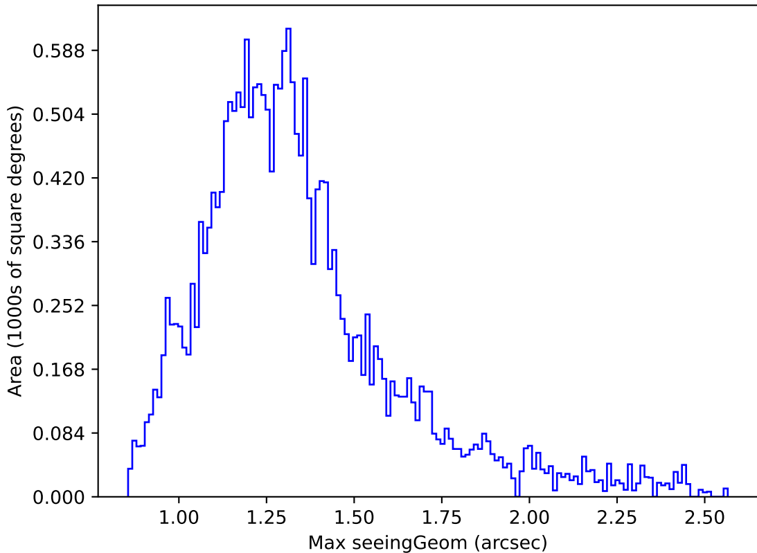
ddf_acor_sf15_lsf40_lsr20_v3.4_10yrs Yr 1 u band: Max seeingGeom
