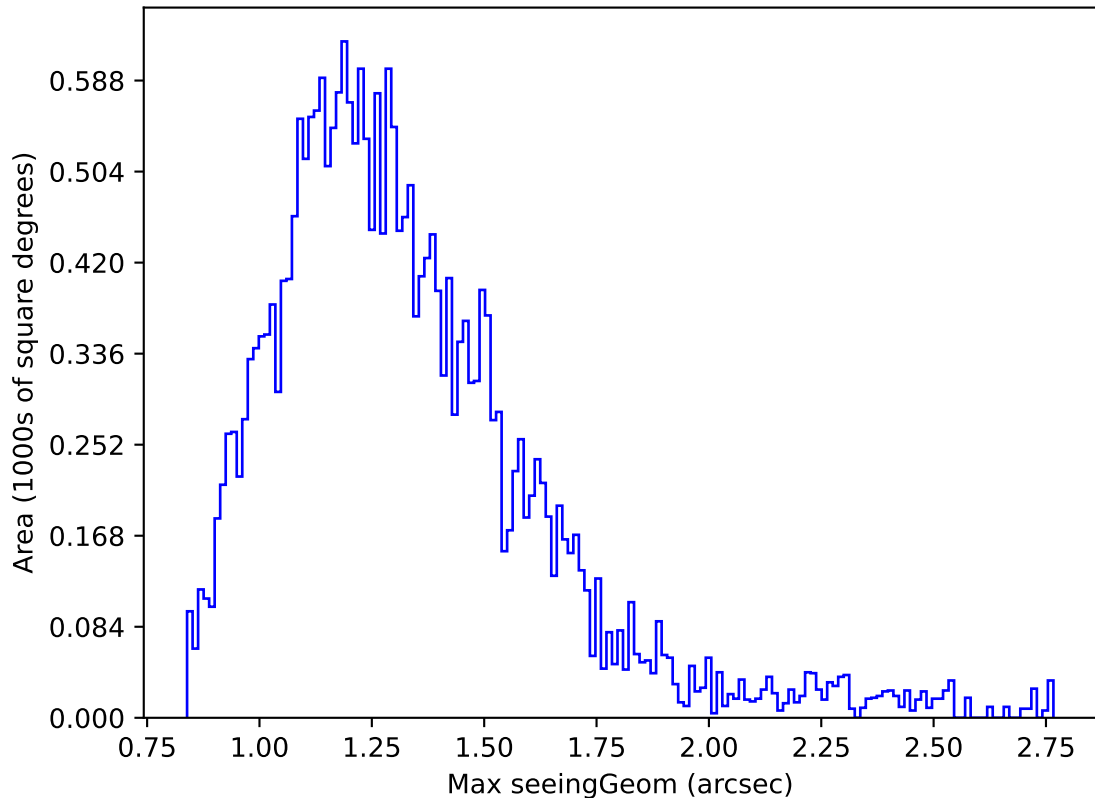
ddf_acor_sf15_ls40_lsr20_v3.4_10yrs Yr 1 i band: Max seeingGeom
