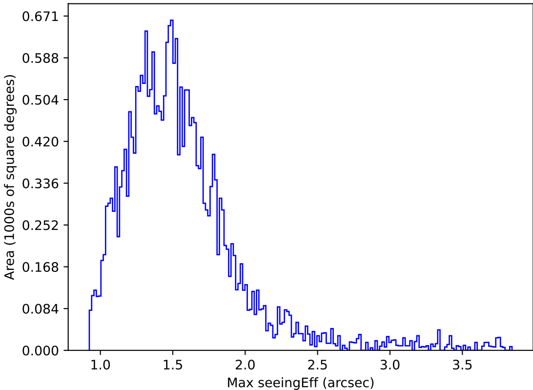
ddf_acor_sf15_lsf40_lsr20_v3.4_10yrs Yr 1 g band: Max seeingEff
