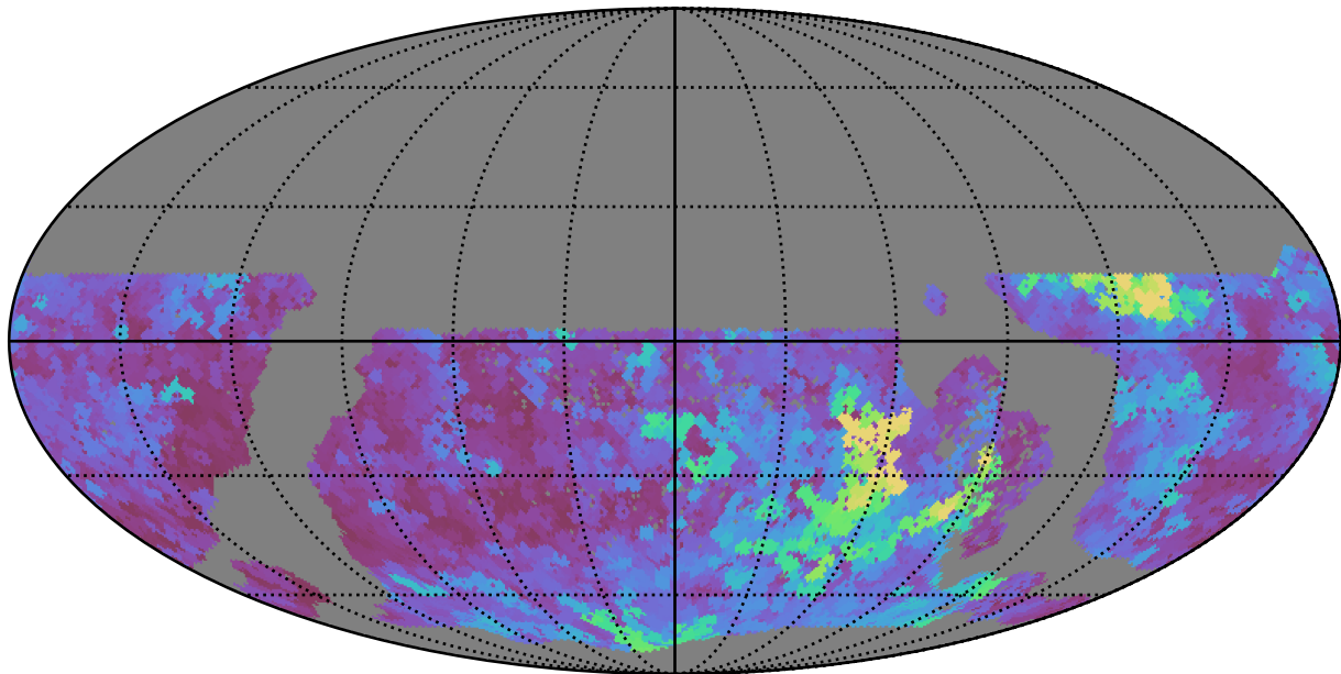
ddf_acor_sf15_lsf40_lsr20_v3.4_10yrs WFD y band: Max seeingEff
