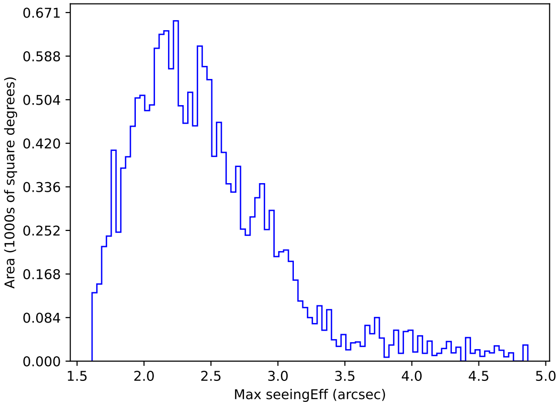
ddf_acor_sf15_lsf40_lsr20_v3.4_10yrs WFD y band: Max seeingEff
