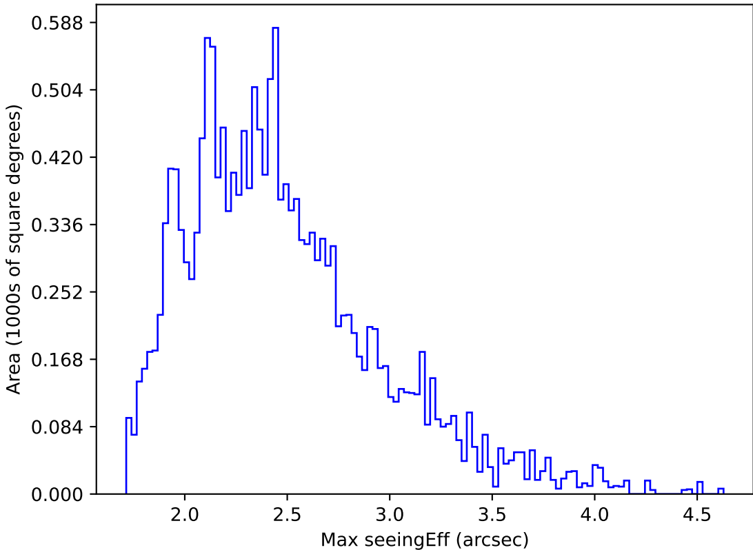
ddf_acor_sf15_lsf40_lsr20_v3.4_10yrs WFD u band: Max seeingEff
