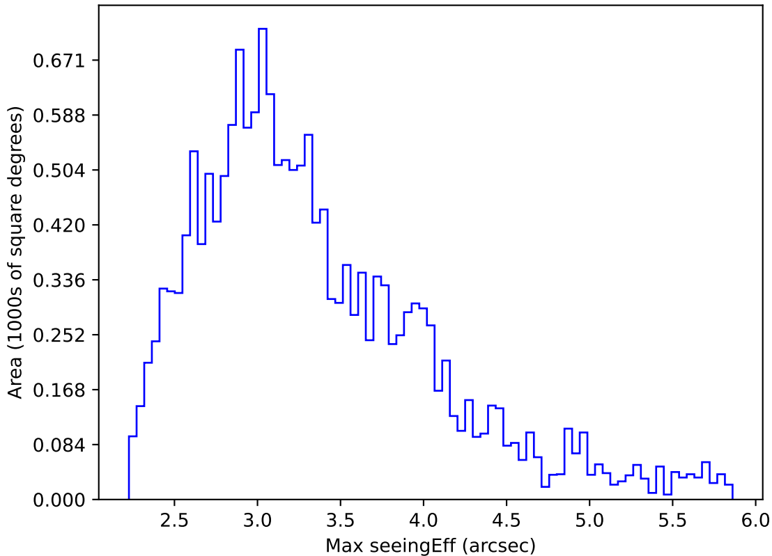
ddf_acor_sf15_lsf40_lsr20_v3.4_10yrs WFD all bands: Max seeingEff
