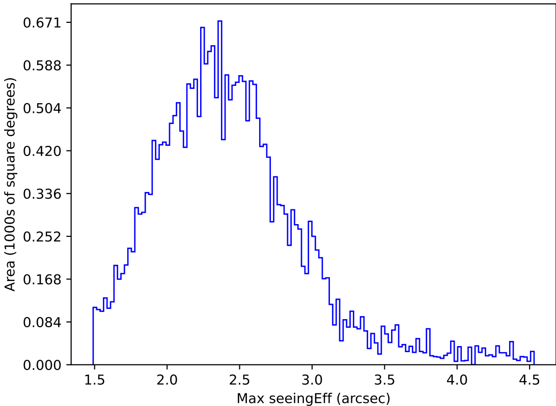
ddf_acor_sf15_lsf40_lsr20_v3.4_10yrs All sky z band: Max seeingEff
