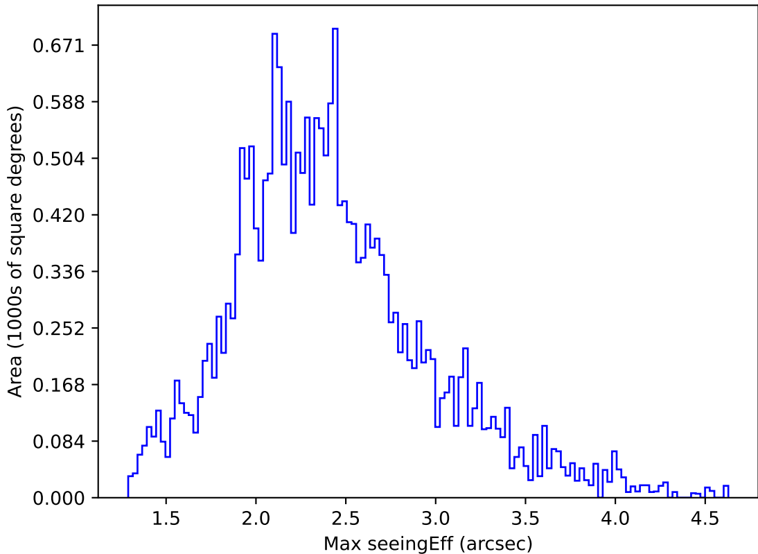
ddf_acor_sf15_ls40_lsr20_v3.4_10yrs All sky u band: Max seeingEff
