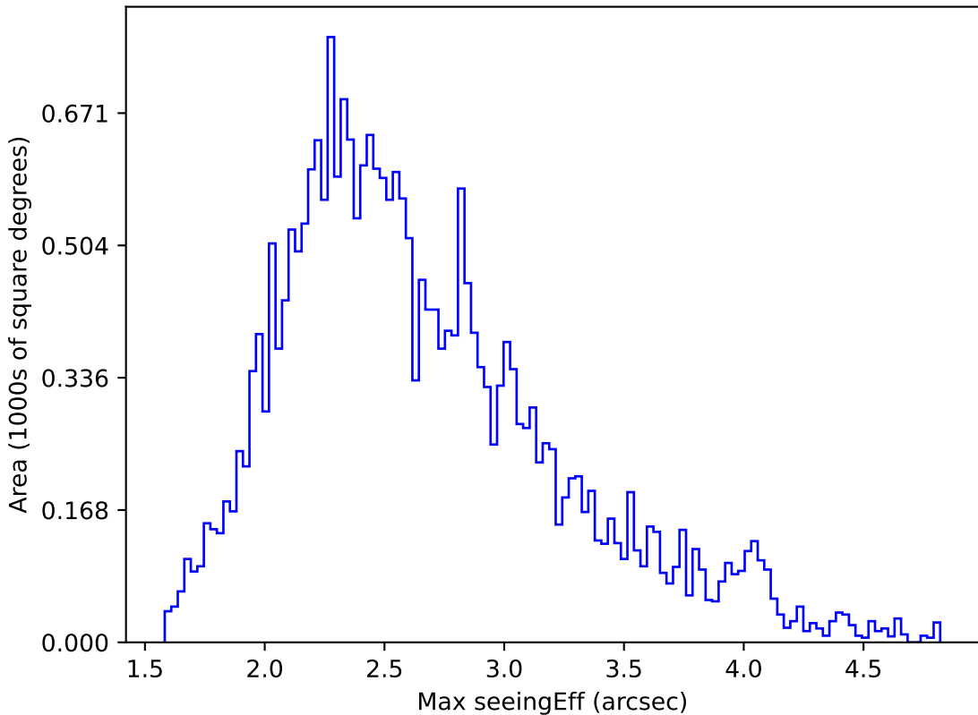
ddf_acor_sf15_lsf40_lsr20_v3.4_10yrs All sky r band: Max seeingEff
