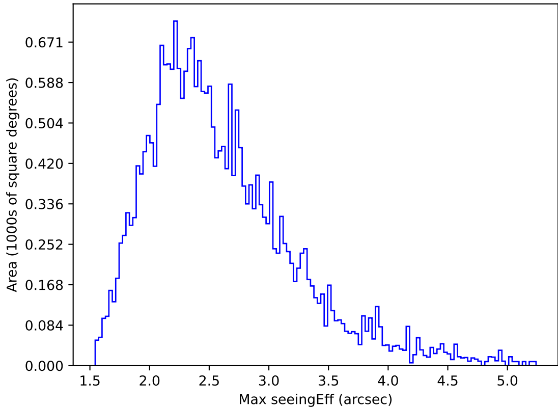
ddf_acor_sf15_lsf40_lsr20_v3.4_10yrs All sky i band: Max seeingEff
