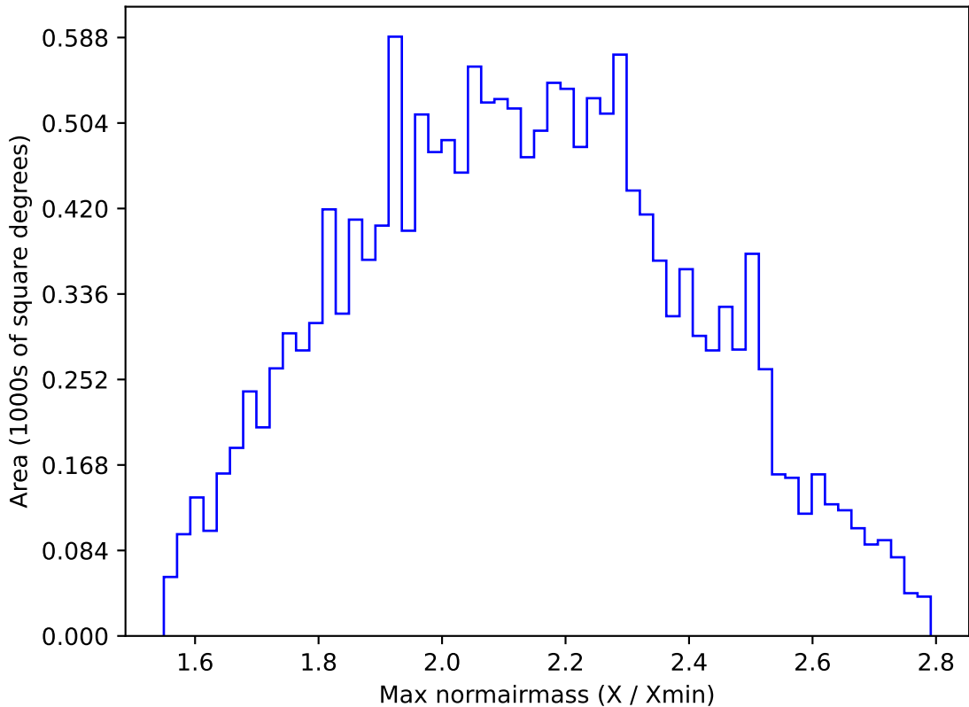
ddf_acor_sf15_lsf40_lsr20_v3.4_10yrs WFD y band: Max normairmass
