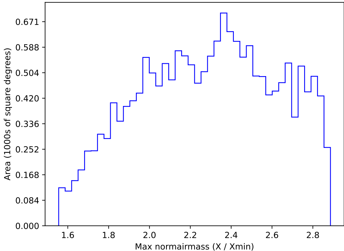
ddf_acor_sf15_lsf40_lsr20_v3.4_10yrs WFD i band: Max normairmass
