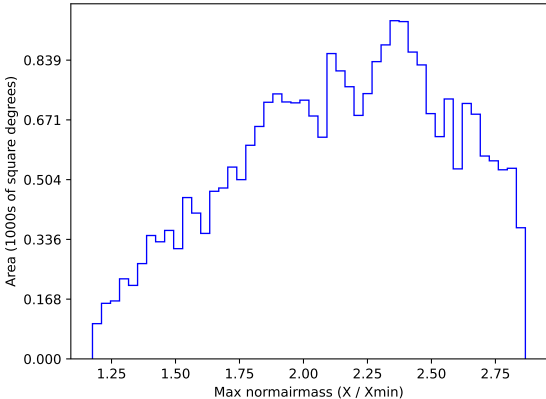
ddf_acor_sf15_ls40_lsr20_v3.4_10yrs All sky z band: Max normairmass
