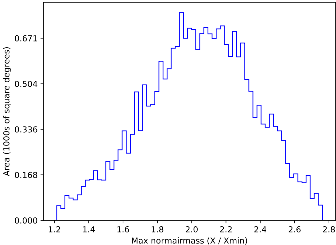
ddf_acor_sf15_lsf40_lsr20_v3.4_10yrs All sky y band: Max normairmass
