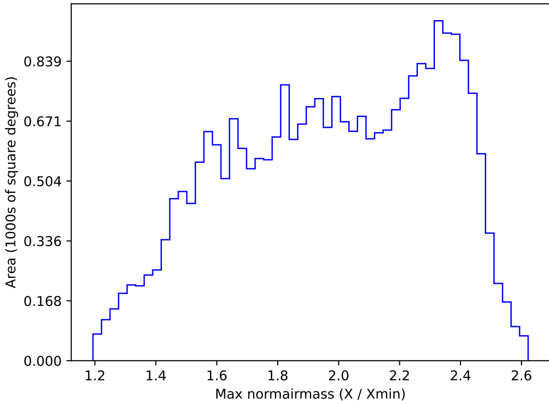
ddf_acor_sf15_ls40_lsr20_v3.4_10yrs All sky r band: Max normairmass
