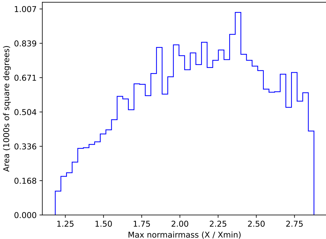
ddf_acor_sf15_lsf40_lsr20_v3.4_10yrs All sky i band: Max normairmass
