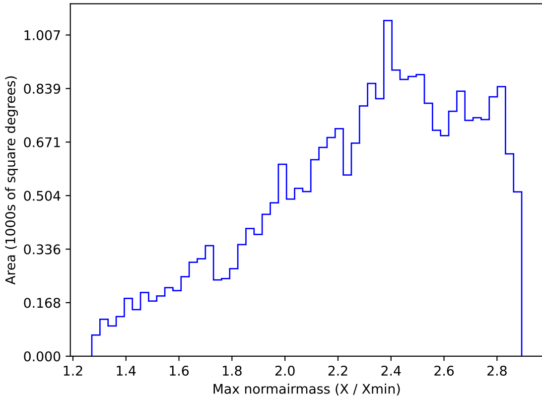
ddf_acor_sf15_lsf40_lsr20_v3.4_10yrs All sky all bands: Max normairmass
