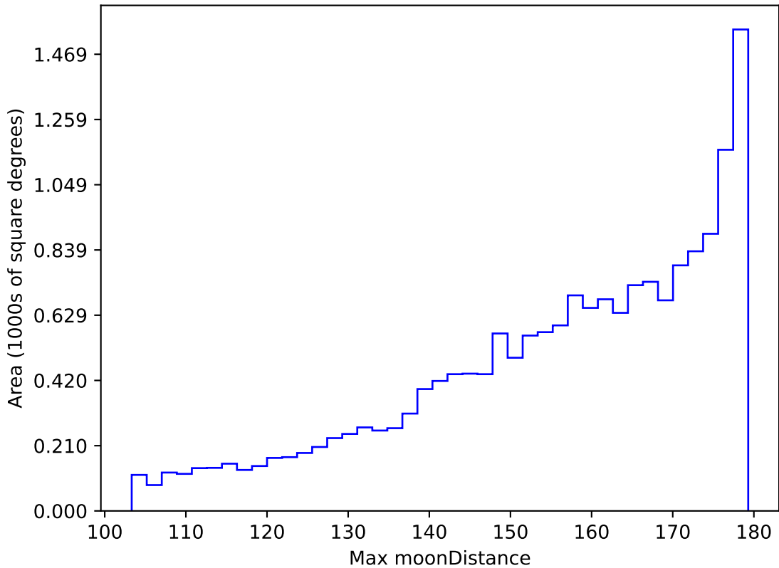
ddf_acor_sf15_lsf40_lsr20_v3.4_10yrs WFD r band: Max moonDistance
