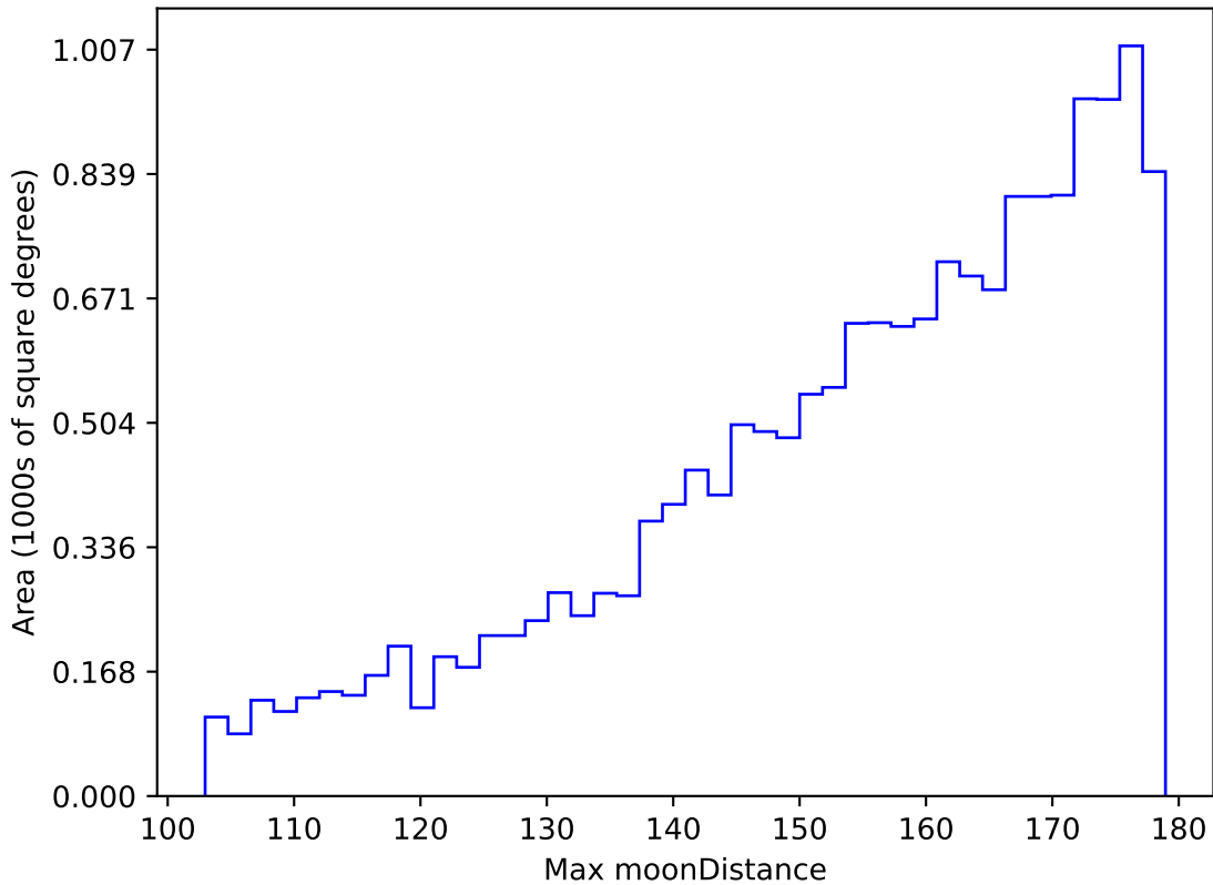
ddf_acor_sf15_lsf40_lsr20_v3.4_10yrs WFD g band: Max moonDistance
