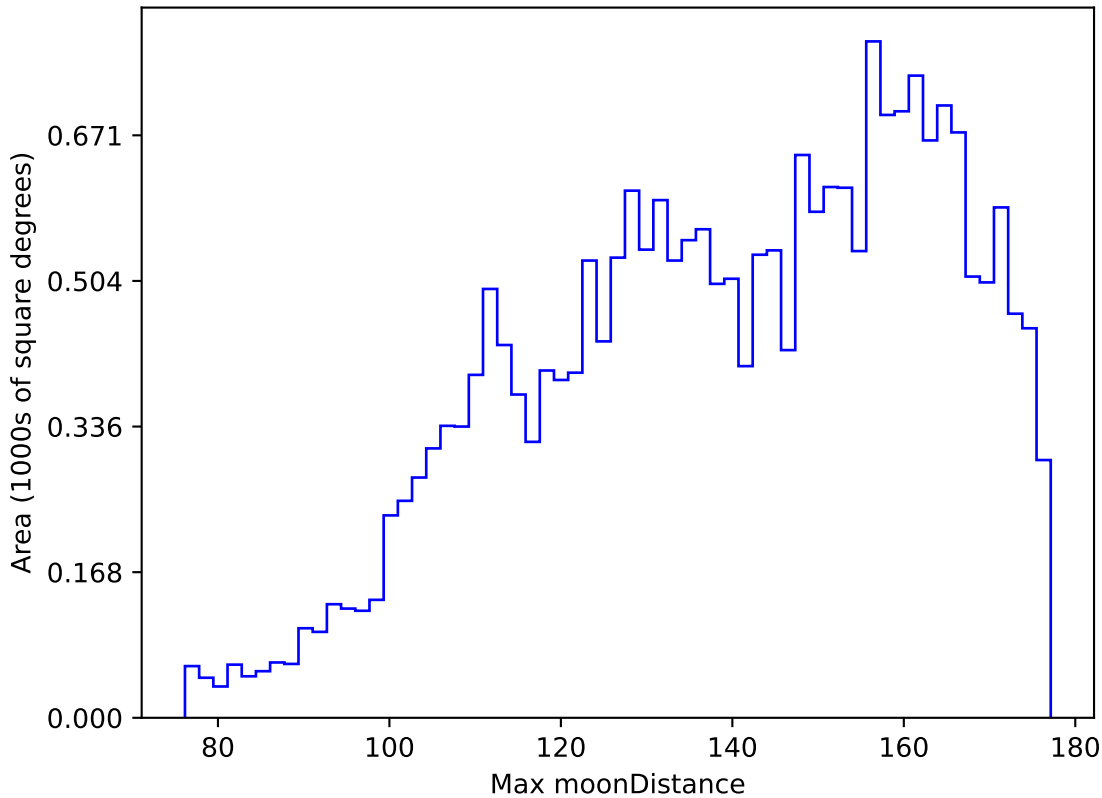
ddf_acor_sf15_lsf40_lsr20_v3.4_10yrs All sky y band: Max moonDistance
