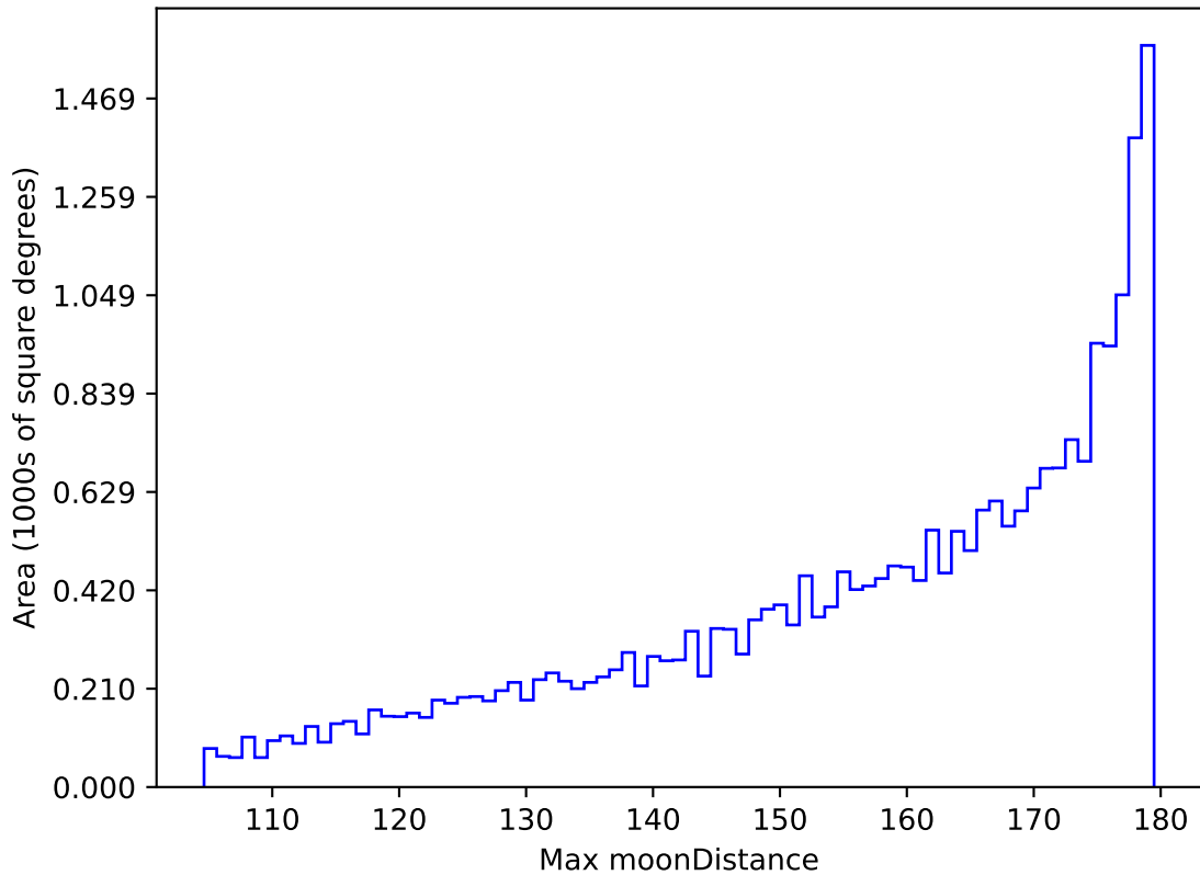
ddf_acor_sf15_lsf40_lsr20_v3.4_10yrs All sky all bands: Max moonDistance
