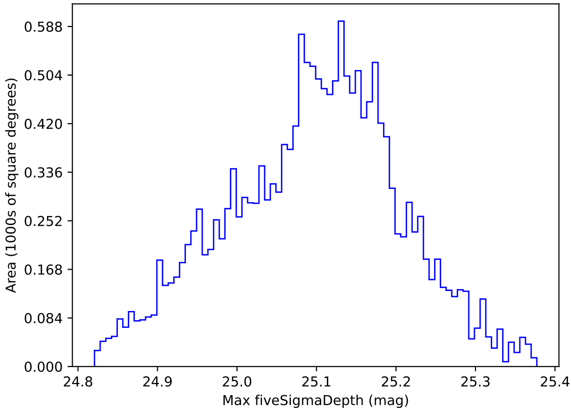
ddf_acor_sf15_lsf40_lsr20_v3.4_10yrs WFD g band: Max fiveSigmaDepth
