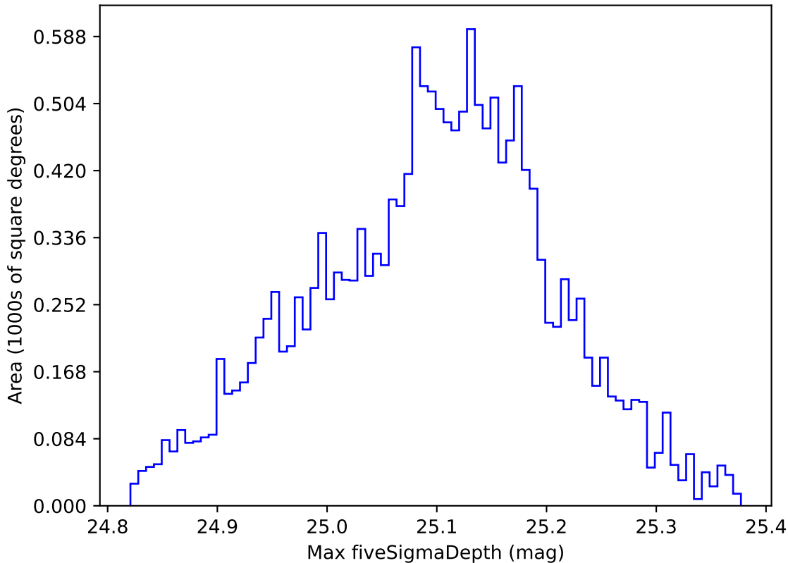
ddf_acor_sf15_lsf40_lsr20_v3.4_10yrs WFD all bands: Max fiveSigmaDepth
