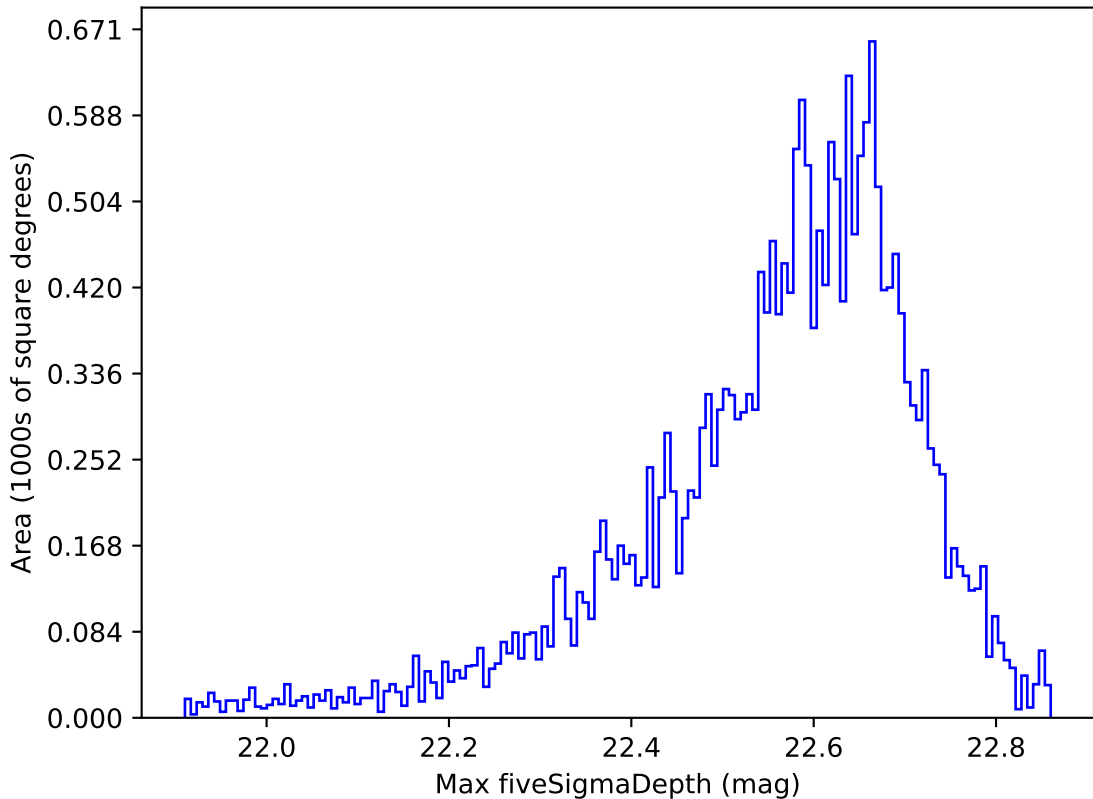
ddf_acor_sf15_ls40_lsr20_v3.4_10yrs All sky y band: Max fiveSigmaDepth
