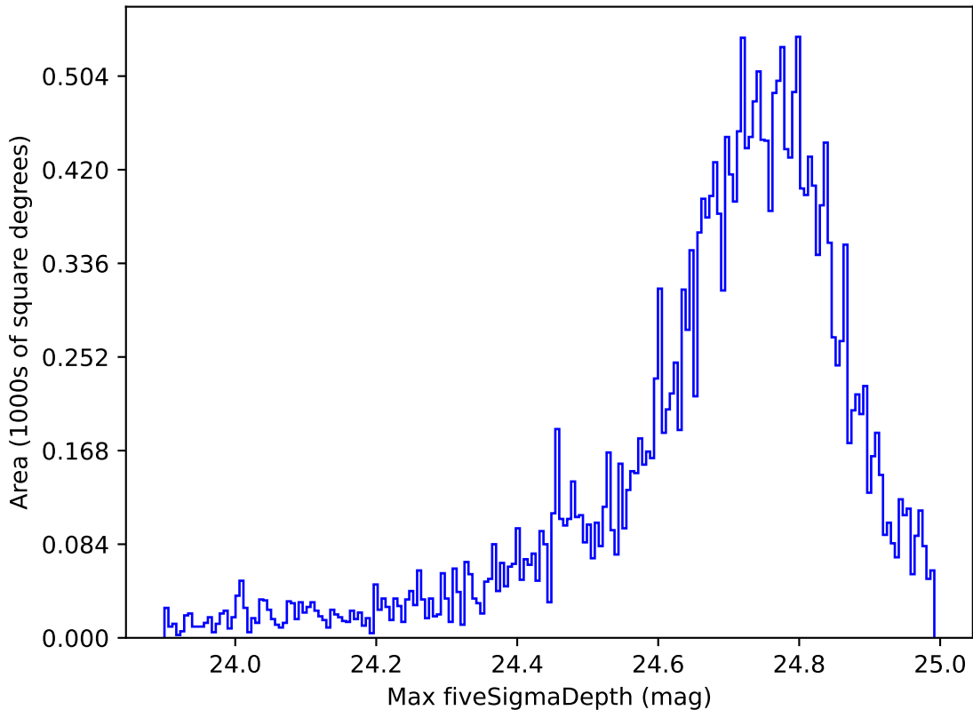
ddf_acor_sf15_lsf40_lsr20_v3.4_10yrs All sky r band: Max fiveSigmaDepth
