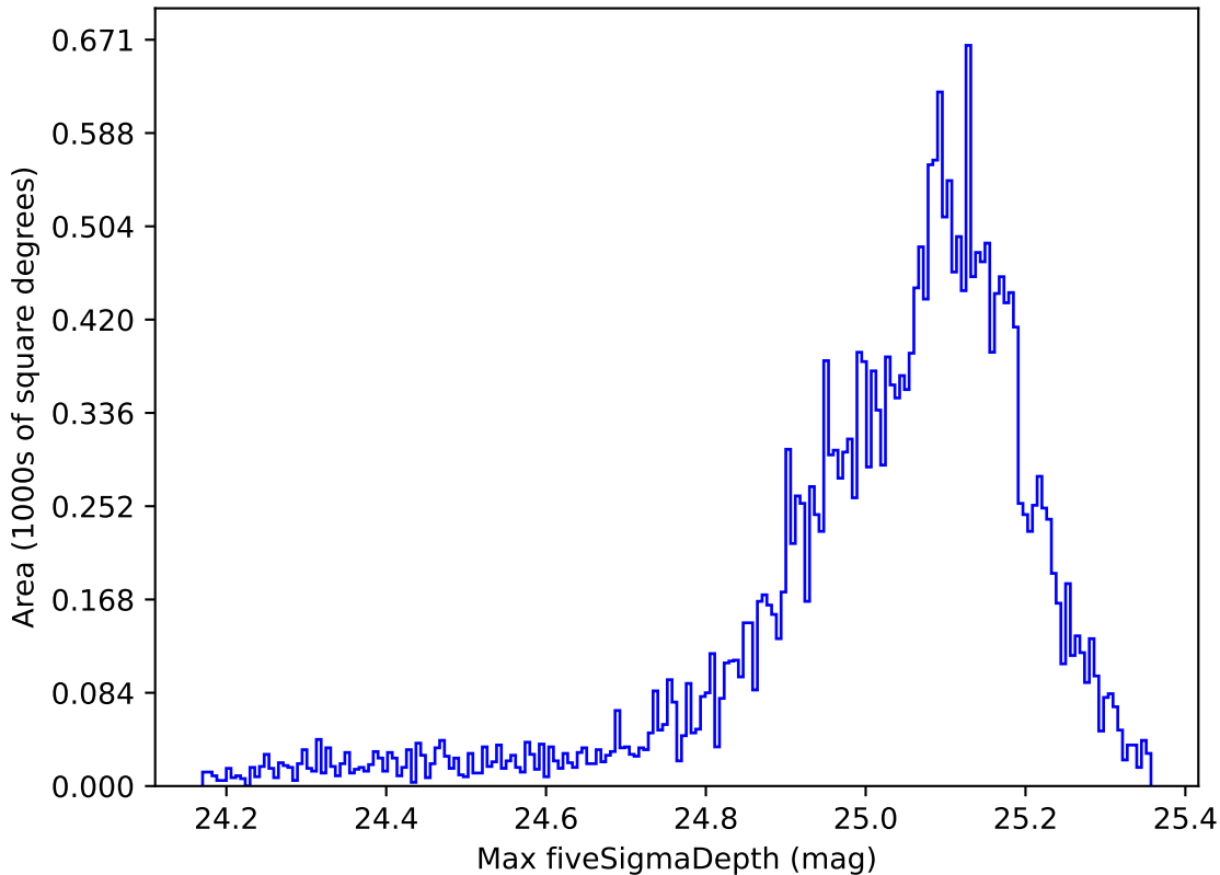
ddf_acor_sf15_lsf40_lsr20_v3.4_10yrs All sky g band: Max fiveSigmaDepth
